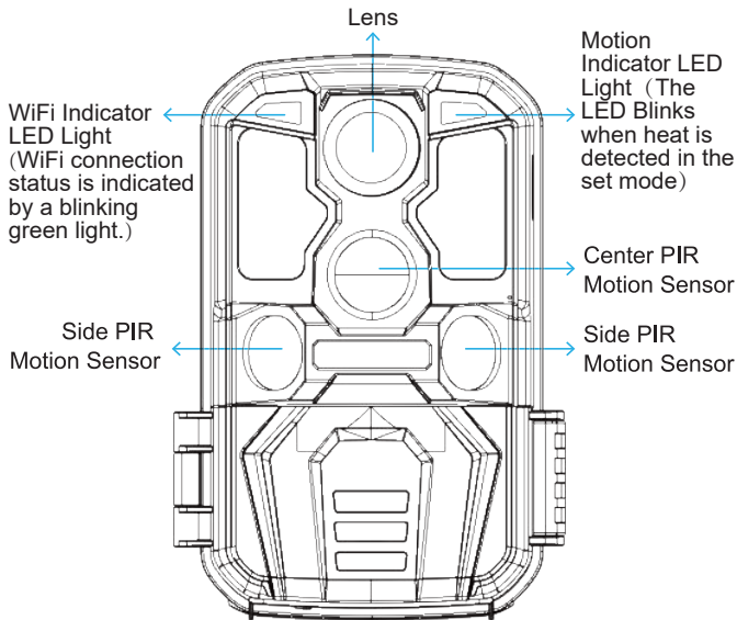
Figure 1: Front View
